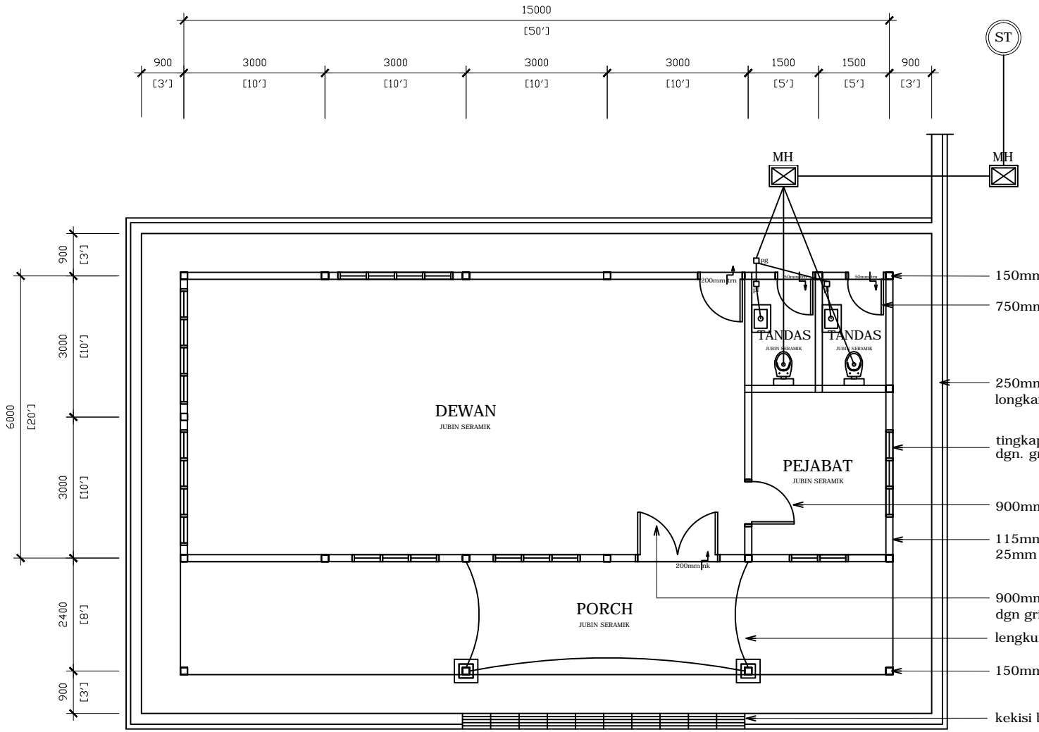
FLOOR PLAN
